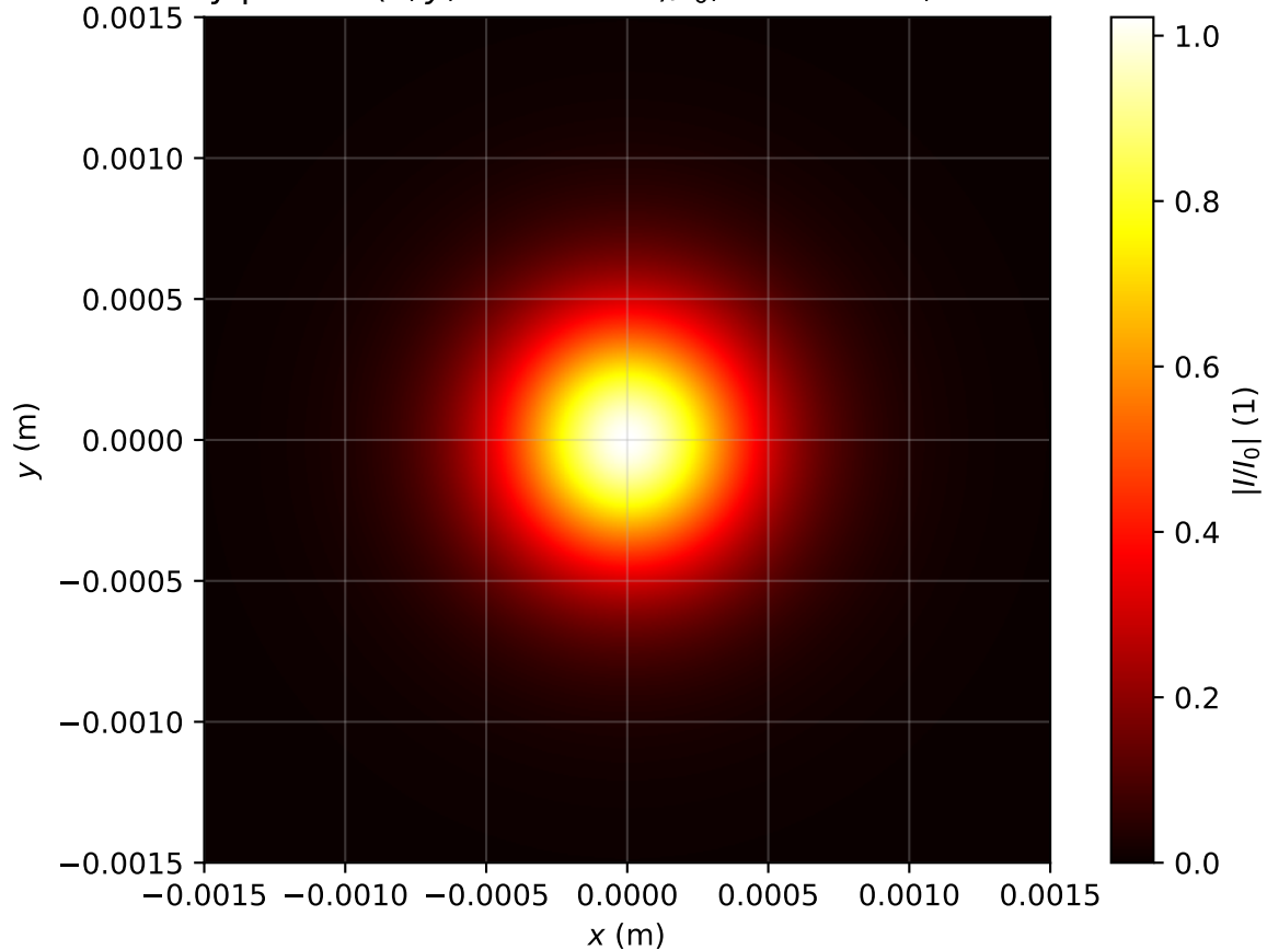
Intensity profile I(x, y, z = 2.309m)/I_0 , Pin=0.7Pcr, artificial time
